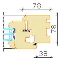
Openable window
