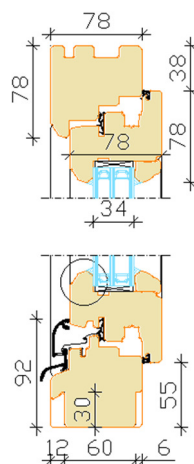
Openable window
