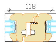
Section without mullion Secondary sash/Primary sash
