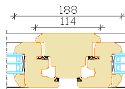
Section through fixed mullion Opening sash/Opening sash
