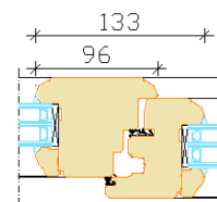
Section through mullion Fixed light / Opening sash
