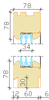
Fixed window
