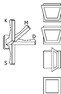
K - Tilt position (ventilation)
