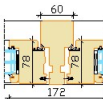
Openable+Openable
