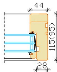
Fixed window
