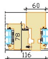
Openable+Fixed
