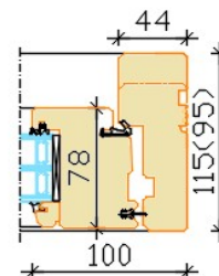
Openable window
