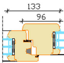
Section through mullion Opening sash /Fixed light
