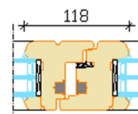
Section without mullion Secondary sash/Primary sash
