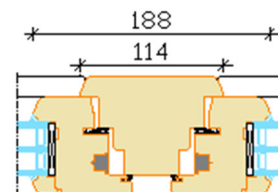
Section through fixed mullion Opening sash/Opening sash
