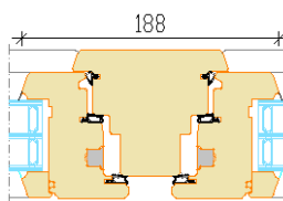
Section through fixed mullion Opening sash/Opening sash
