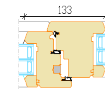
Section through mullion Opening sash /Fixed light
