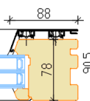
Fixed window
