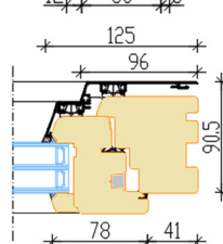
Operable window
