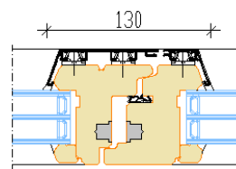
Section without mullion Secondary sash/Primary sash
