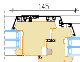
Section through mullion Opening sash /Fixed light
