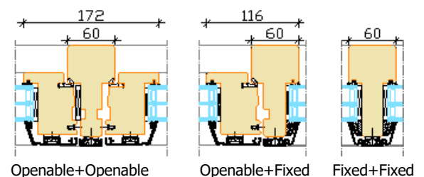
Openable+Openable
