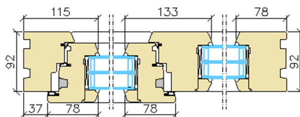
Sliding part
