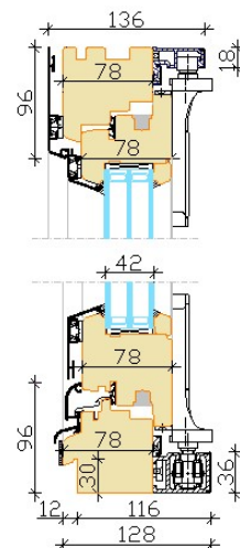
Vertical section With standard wooden threshold
