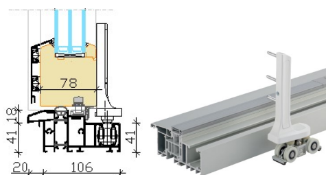
Komfort threshold and lower roller
