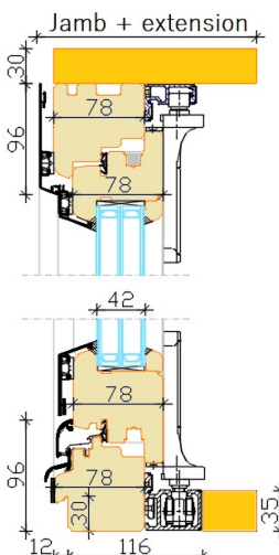
Extension of jamb
