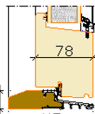
Combi threshold
