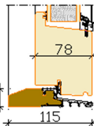
Combi threshold
