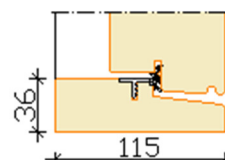
Oak threshold
